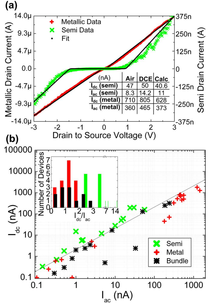
FIG. 2. (Color online) (a) Drain current ( I_{ds} ) as a function of drain to source voltage ( V_{ds} ) for a typical semiconducting and a metallic carbon nanotube. Measured data and the associated fit to Eq. (2) are shown. (b) Distribution of I_{ac} and I_{dc} values for 43 representative nanotube devices. Inset shows histogram binning of the I_{dc}/I_{ac} ratio.
